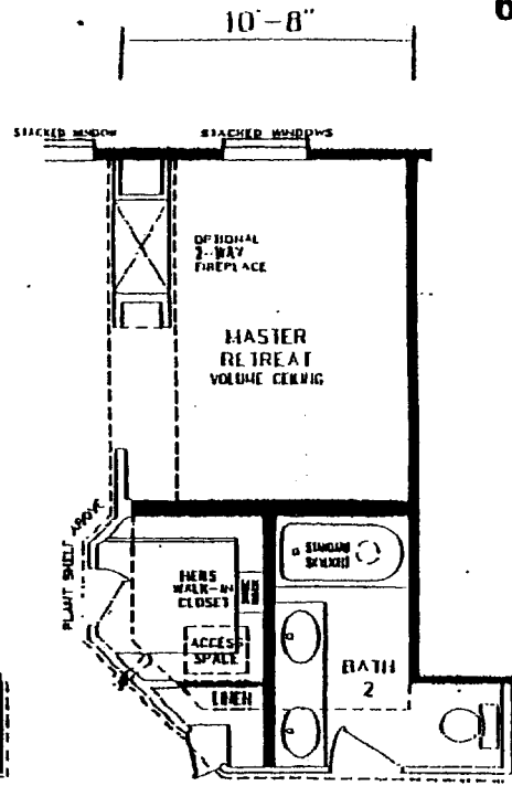
MASTER RETREAT WITH OPTIONAL TWO-WAY FIREPLACE
